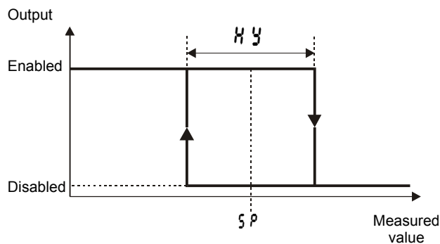
Fig. 16. Operation way of the heating output type
